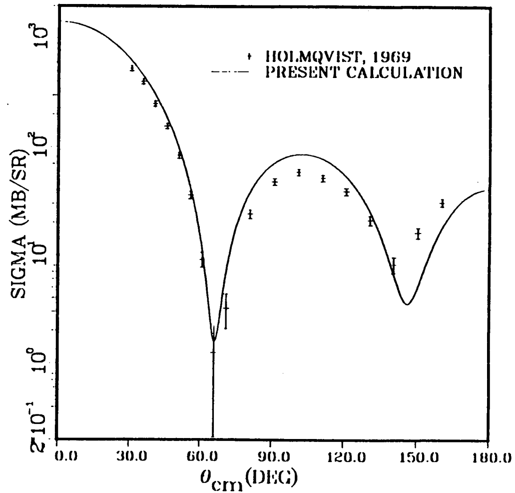
Figure 4.14 Comparison of Theoretical and Experimental Values Obtained for ^{64}\text{Zn} + n Elastic with E_N = 3.44 MeV
