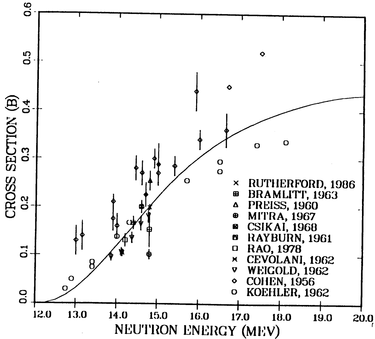
Figure 5.1 Comparison of Experimental and Theoretical Values of ^{64}\text{Zn}(n, 2n)^{63}\text{Zn} Cross Sections from 12.0 - 20.0 MeV
