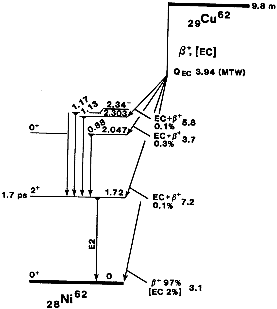
Figure 3.4 Decay Scheme of ^{29}\text{Cu}^{62}
