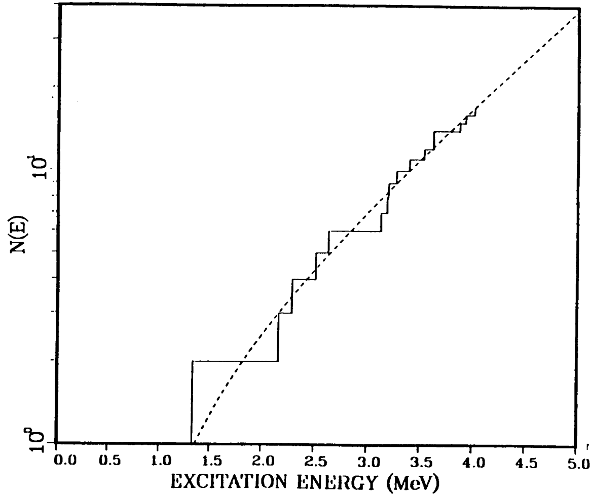
Figure 4.11 Experimental Levels and Level Fit of ^{60}\text{Ni}
