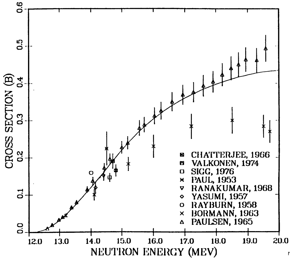
Figure 5.2 Comparison of Experimental and Theoretical Values of ^{64}\text{Zn}(n, 2n)^{63}\text{Zn} Cross Sections from 12.0 - 20.0 MeV
