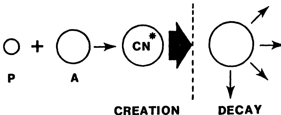
Figure 4.12 Schematic Illustration of Reaction Models
