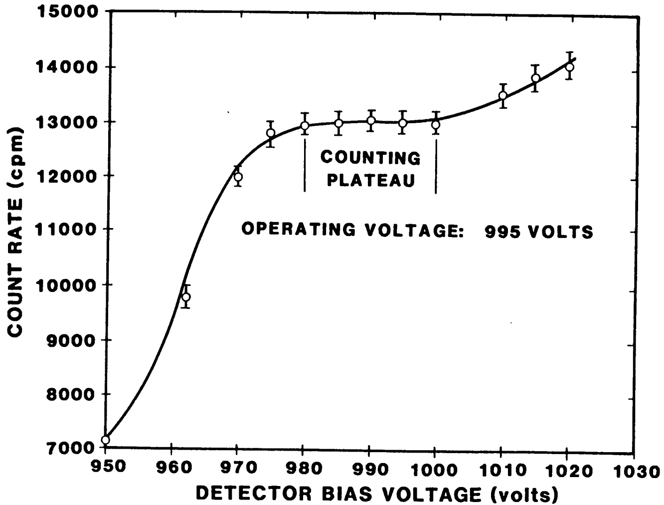
Figure 2.5 Counting Plateau Determination NaI (Tl) Spectrometer Disc. Bias = 0.1 Volts, Source: Na-22
