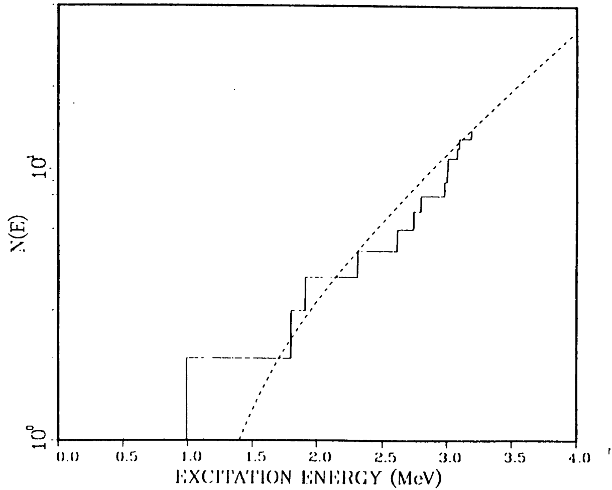
Figure 4.6 Experimental Levels and Level Fit of ^{64}\text{Zn}
