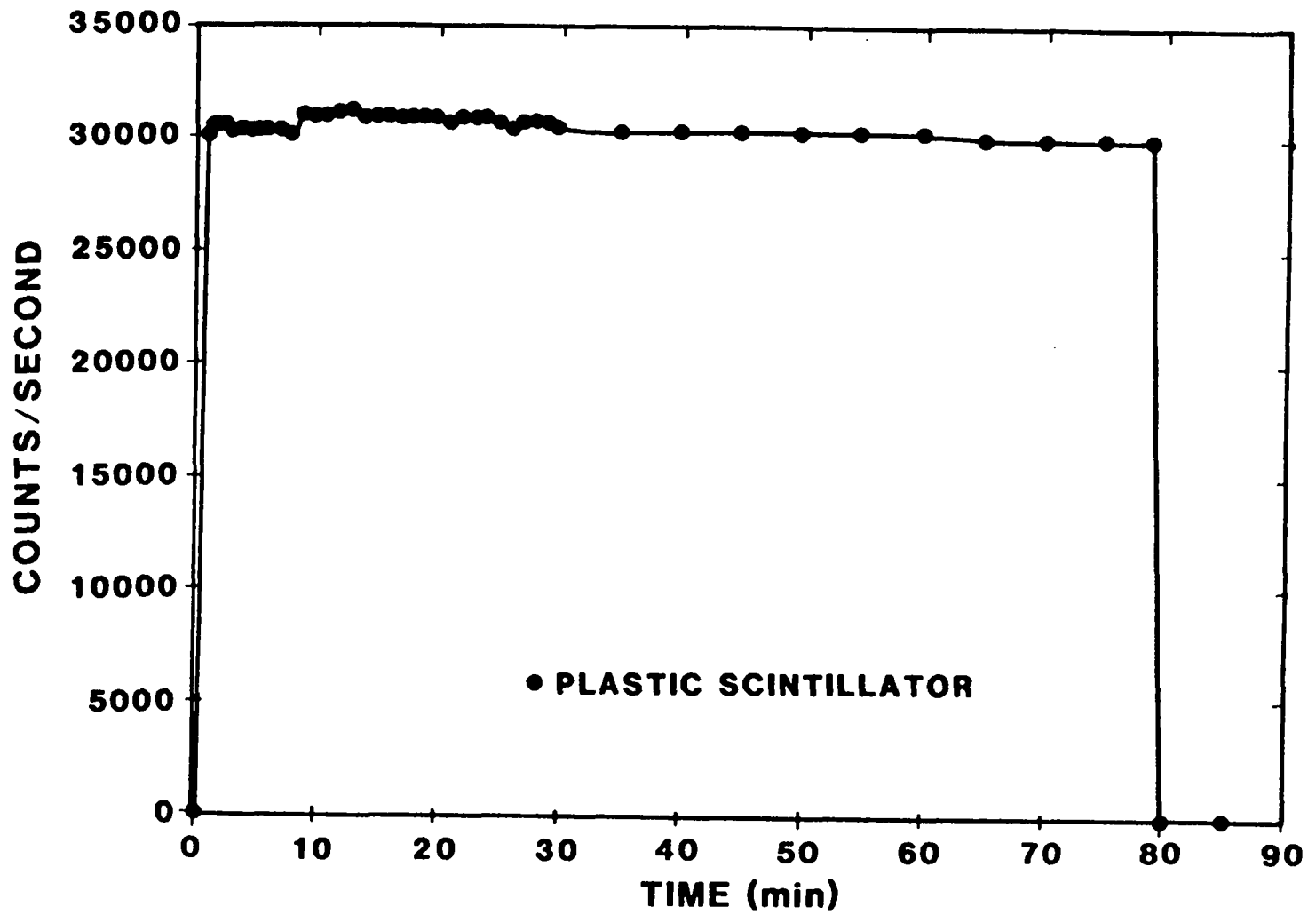
Figure 2.3 Neutron Output as Recorded by the Neutron Monitor (Plastic Scintillator)
