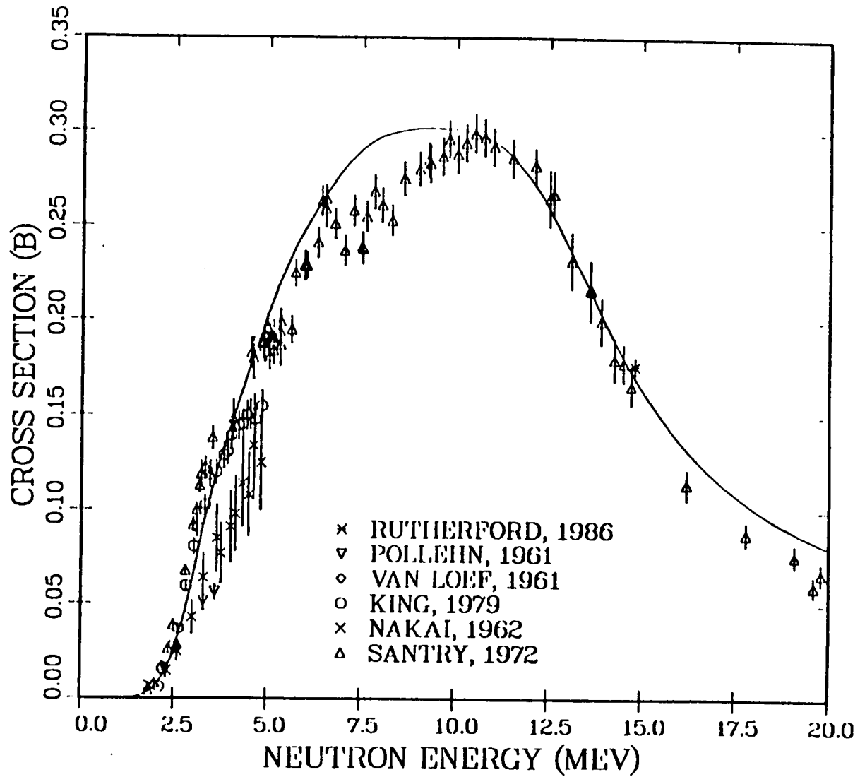
Figure 5.3 Comparison of Experimental and Theoretical Values of ^{64}\text{Zn}(n,p)^{64}\text{Cu} Cross Sections from 0.0 - 20.0 MeV
