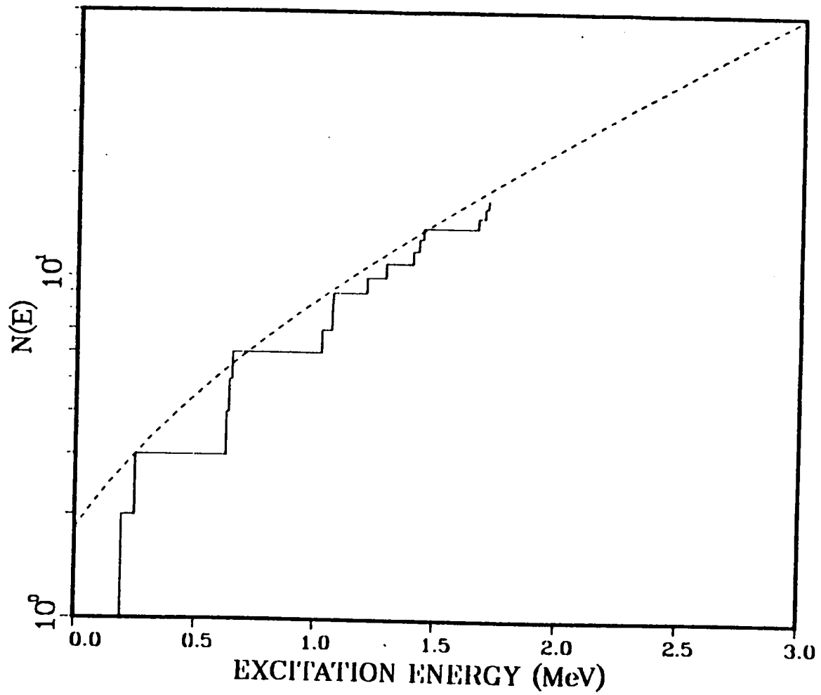
Figure 4.7 Experimental Levels and Level Fit of ^{63}\text{Zn}
