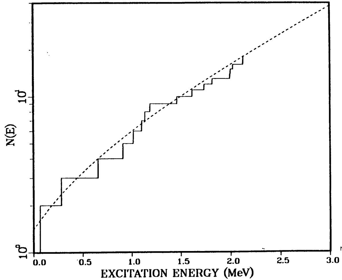
Figure 4.10 Experimental Levels and Level Fit of ^{61}\text{Ni}
