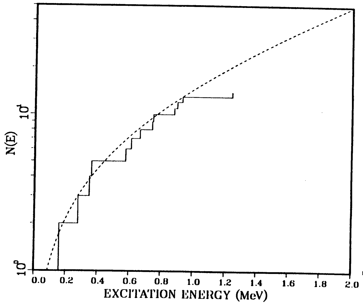
Figure 4.8 Experimental Levels and Level Fit of ^{64}\text{Cu}
