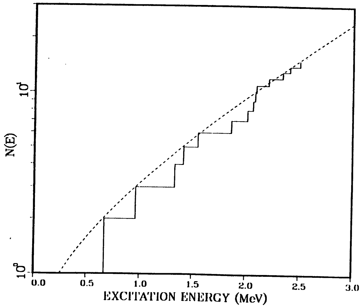
Figure 4.9 Experimental Levels and Level Fit of ^{63}\text{Cu}
