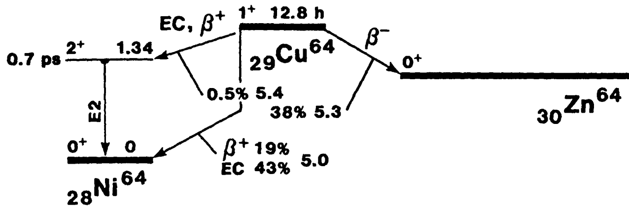
Figure 3.3 Decay Scheme of ^{64}_{29}\text{Cu}
