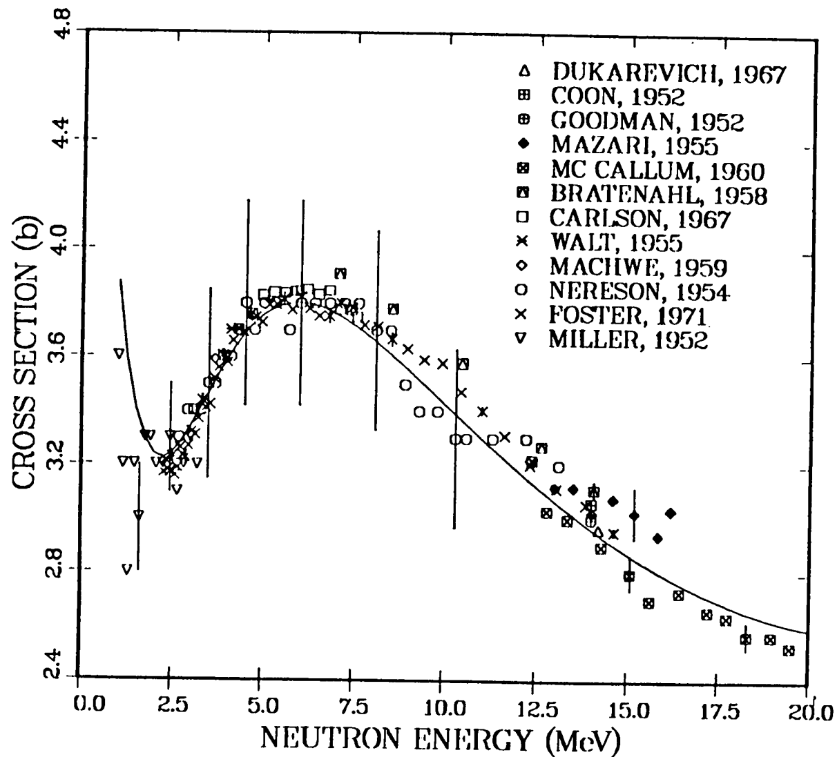
Figure 4.13 Comparison of Theoretical and Experimental Values of n + \text{Zn} Total Cross Sections from 0.0 - 20.0 MeV
