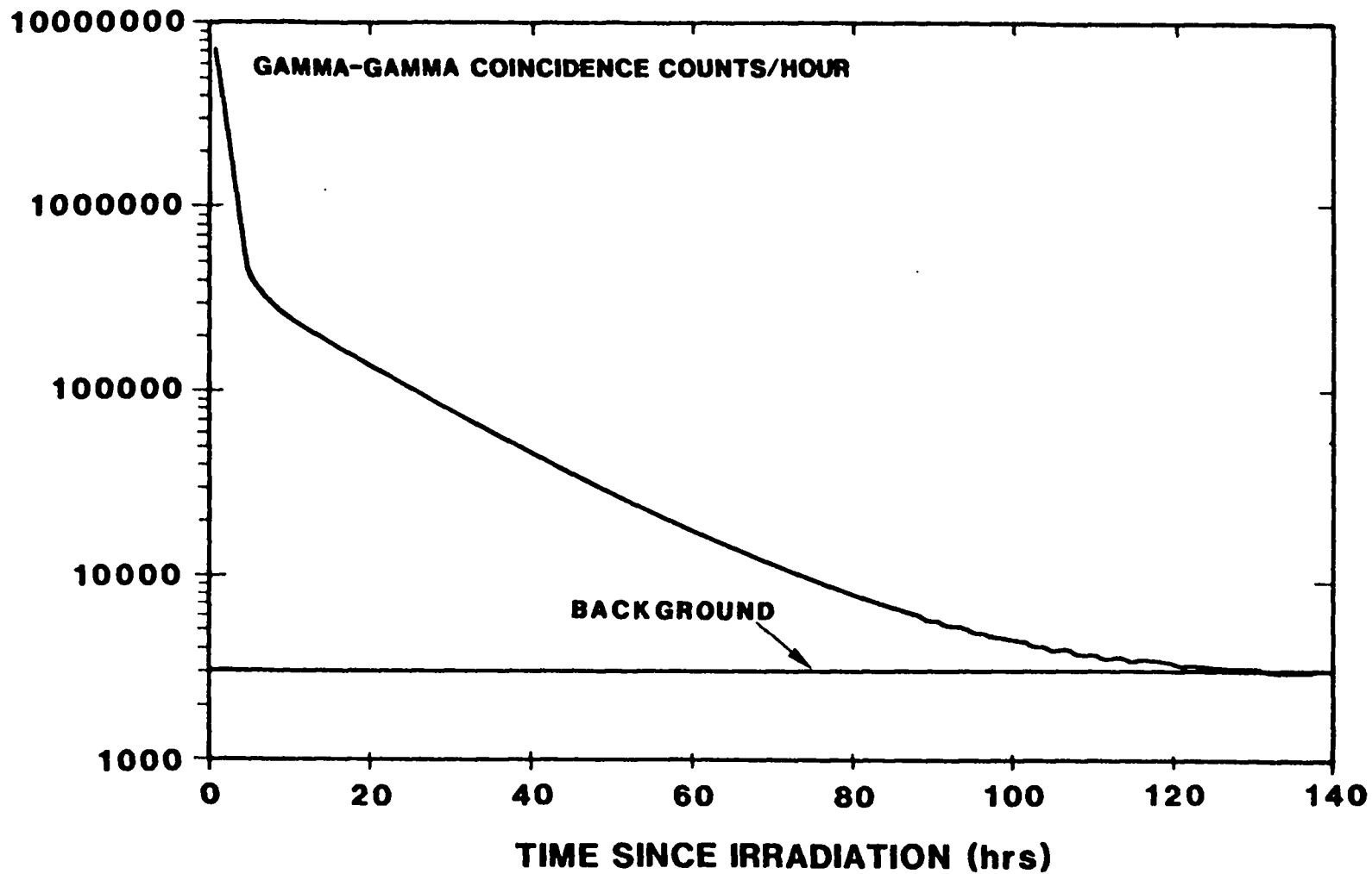
Figure 3.1 Disintegration of Irradiated ^{64}\text{Zn} Foil
