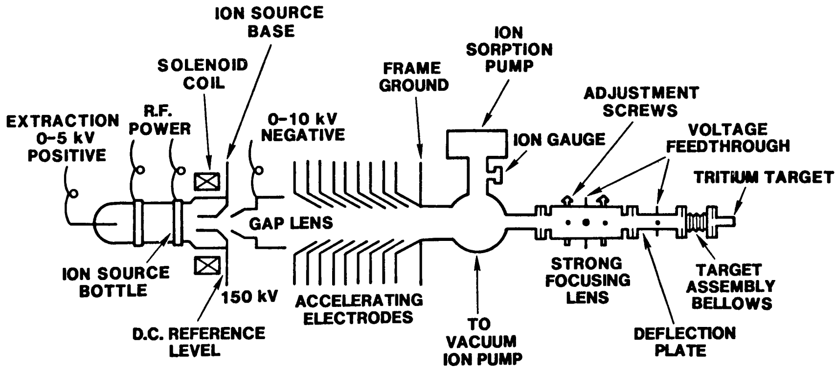
Figure 2.1 Major Components of the Texas Nuclear Neutron Generator
